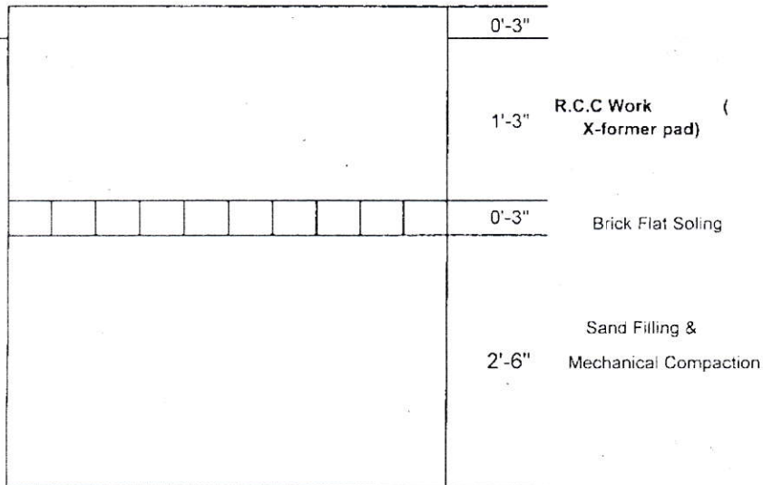
b) Power Transformer Pad Design & Mesurment
