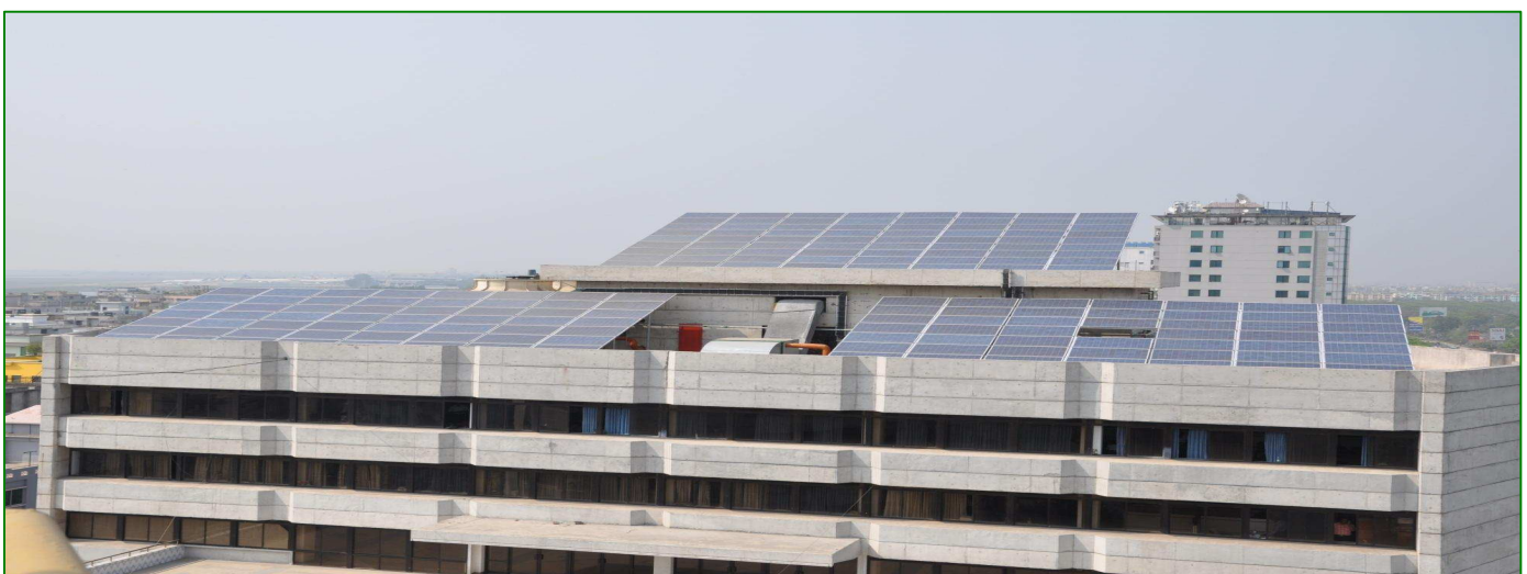
Complete view of 49 kWp Solar Panel
